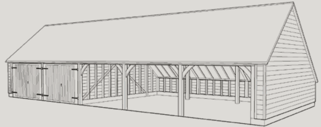
Simple five bay garage with catslide rear roof and two closed bays
